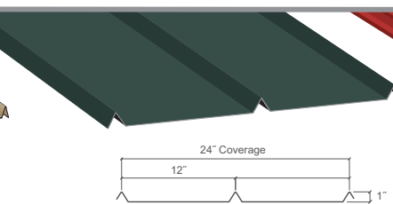
AP Panel
