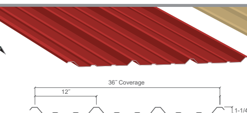
R Panel
